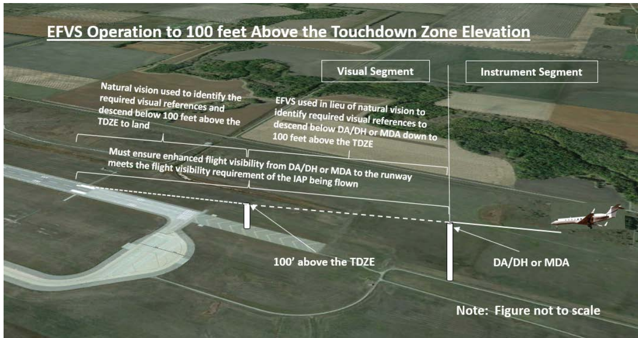
Figure 3. Operational Concept for an EFVS Operation to 100 Feet Above the Touchdown Zone Elevation
